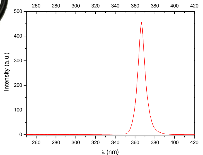
Spectral emission intensity of: UV-Quelle
